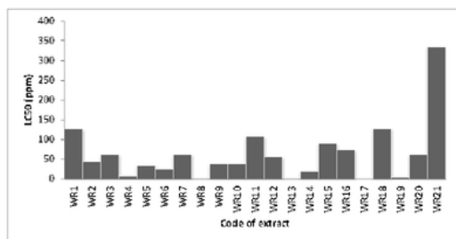
Fig. 1: Brine shrimp toxicity results ( LC_{50} in ppm).
